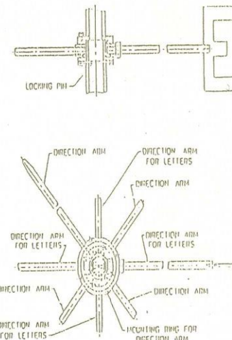
Fig. 62 DETAILS OF ATTACHMENT OF DIRECTION ARMS TO MOUNTING RING OF WINDVANE
