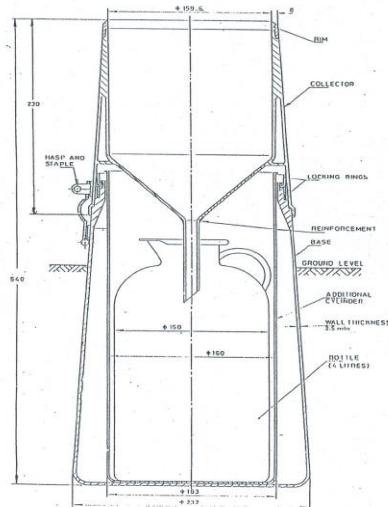
Fig. 14 RAIN GAUGE, Non-Flashed (200 cm 3 ), General Assembly
